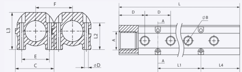
SINGLE DISTRIBUTION MANIFOLD – RED BSSP FEMALE
