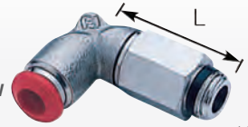
EXTENDED SWIVEL ELBOW WITH NBR90 SEAL RING BSPT MALE
