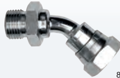
45° SWEEP ELBOW BSPP MALE / BSPP FEMALE
